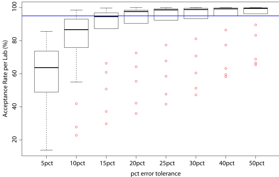
Figure 4 : ION-R variance for the 319,888 positive observations of lorazepam, displayed as the distribution of ION-R acceptance rates/lab at various error tolerances.
